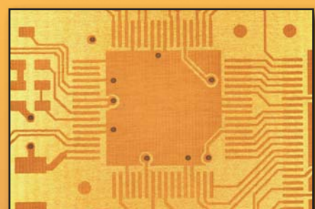
Panel printed with LithoJet 210 Etch Resist
