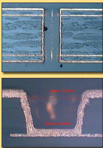
Excellent coverage on both through holes and microvias 通孔與盲孔皆有良好的覆蓋性
