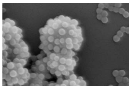
A high power microscopic image of Avanse latex particles adsorbed onto the surface of a titanium dioxide particle
